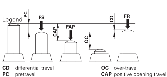
Contacts with single interruption and double contacts
